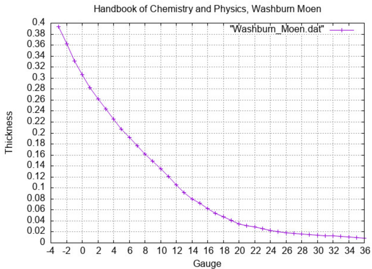
Figure 8: Washburn& Moen
