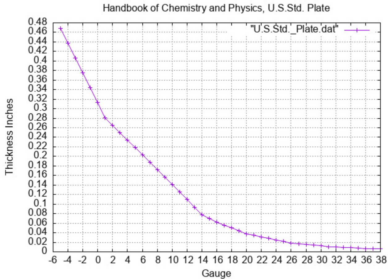
Figure 7: U.S.Std. Plate
