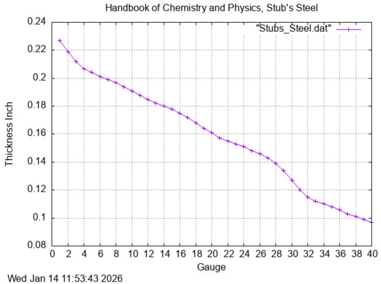
Figure 6: Stubs Steel
