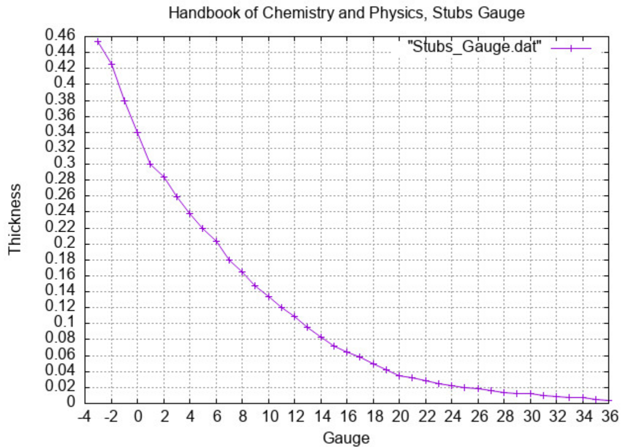
Figure 5: Stubs Gauge
